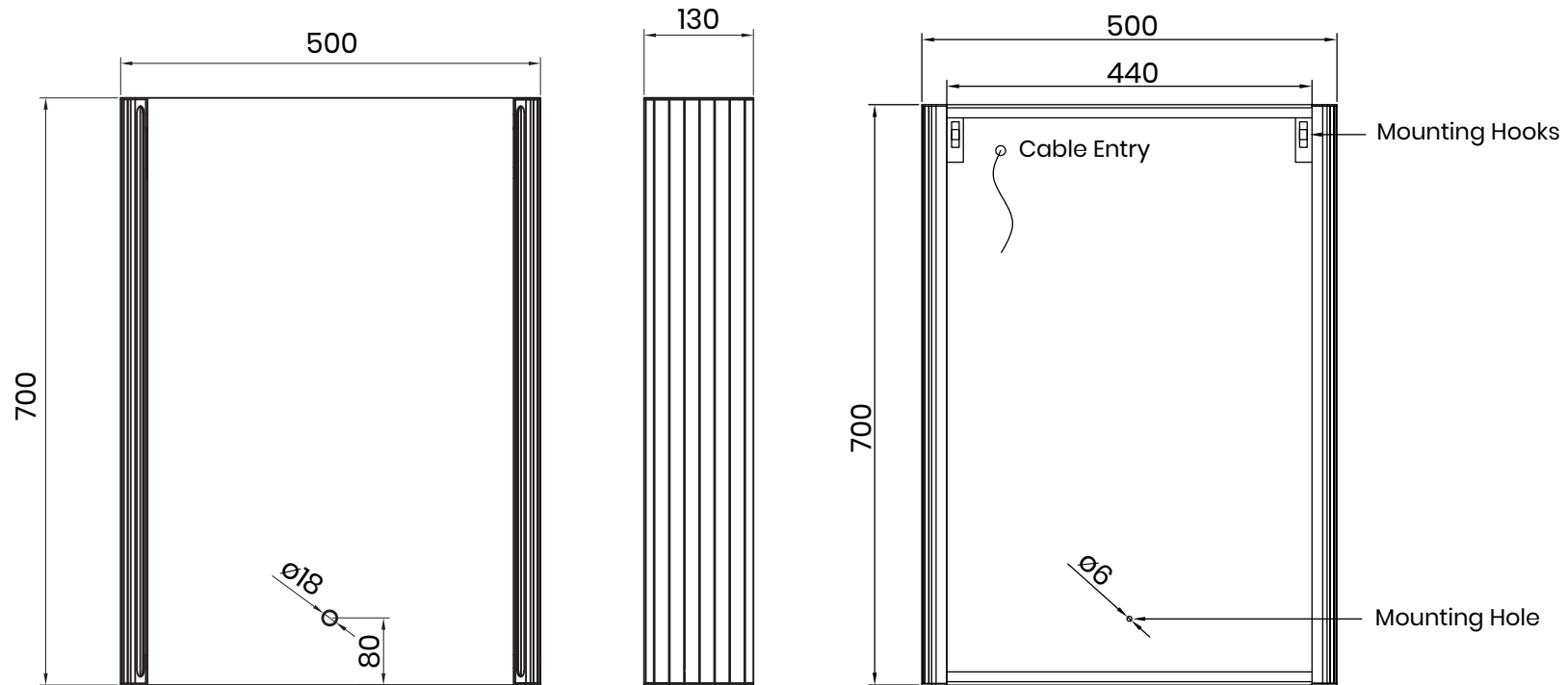
Front View
