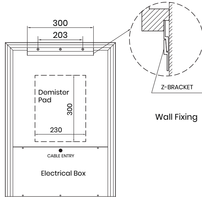
Back View
